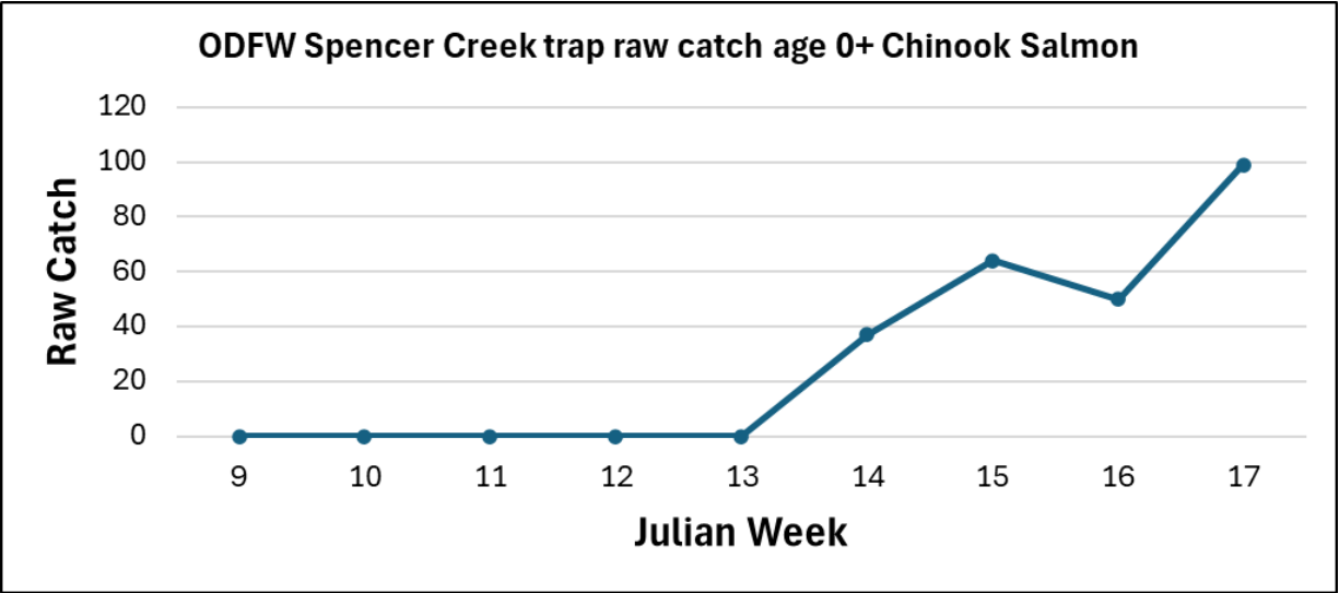
Figure 1. Raw catch of age 0+ Chinook Salmon in the ODFW Spencer Creek fyke trap, summarized by Julian week.
